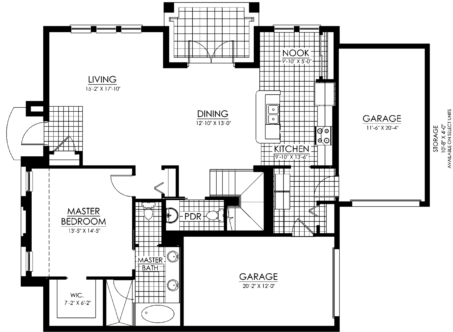
GROUND FLOOR
